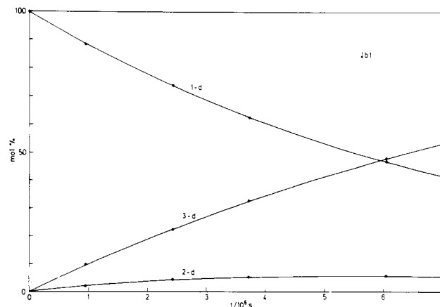
Figure 1. Time dependence of (a) 1-h, 2-h, and 3-h and (b) 1-d, 2-d, and 3-d in methanol with 0.314 M p\text{-NO}_2\text{PhO}^- buffered with 0.674 M p\text{-NO}_2\text{PhOH} at 30.00 \pm 0.03^\circ\text{C} . The curves shown are computer simulated, and the points are the experimentally measured concentrations. Similar curves were obtained with 0.245 M p\text{-NO}_2\text{PhOH} .
